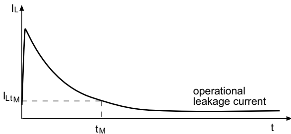
Fig.7: Typical variation with time of the leakage current
