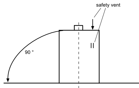
Fig.10 Recommended mounting position
