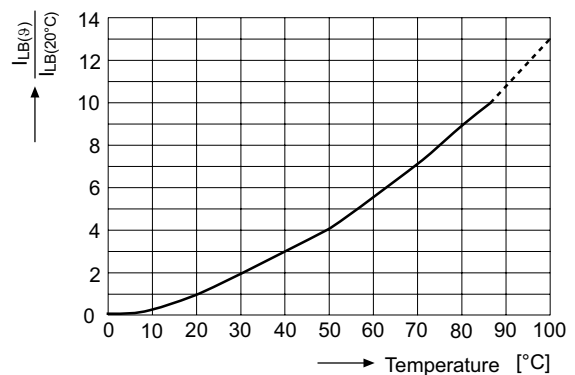
Fig.9 typical variation of leakage current with temperature
